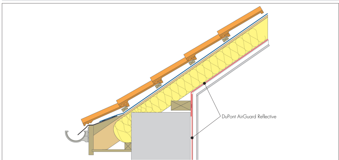
Figure 1 Wall/pitched warm roof detail
